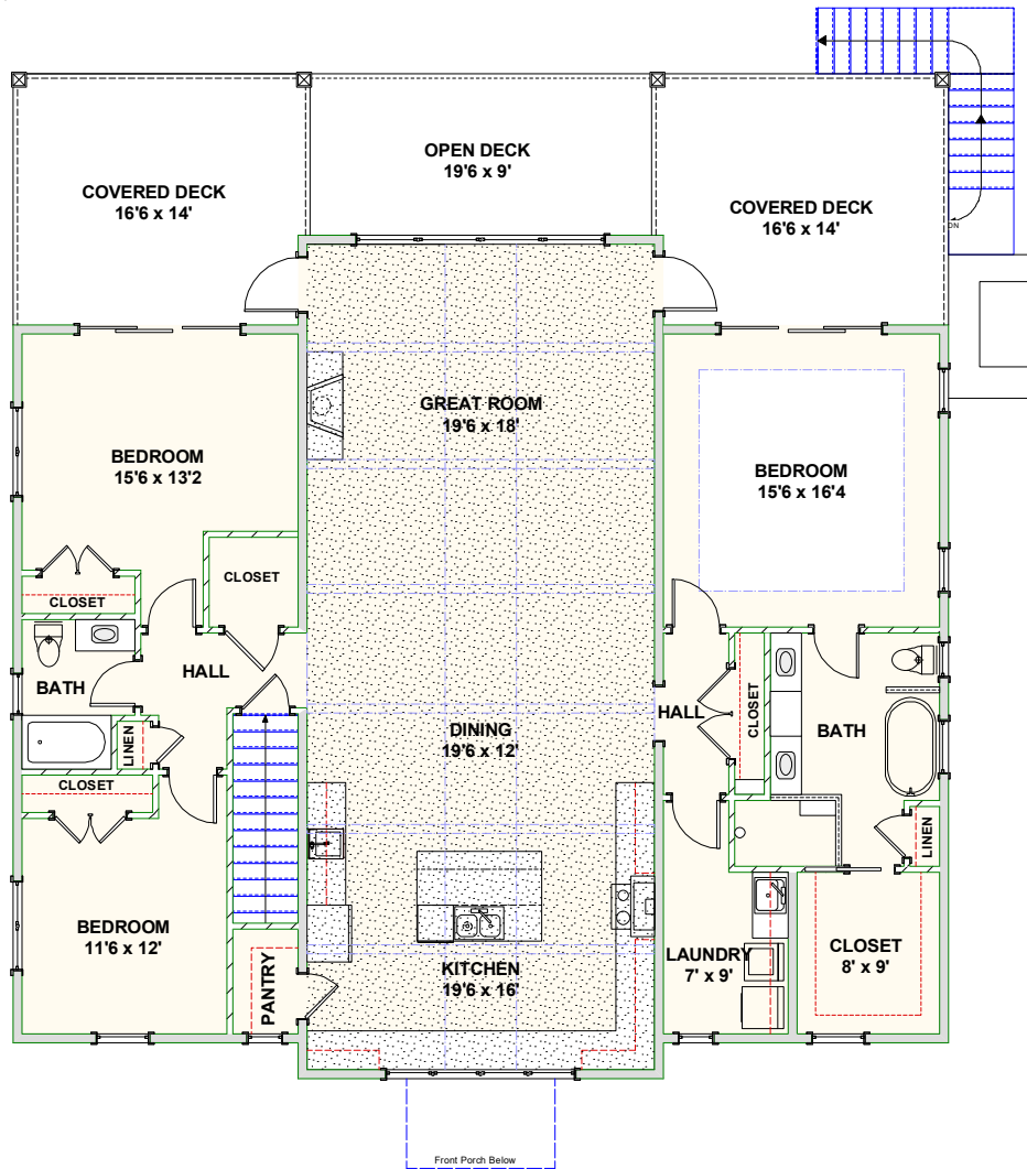
1ST FLOOR - FLOOR PLAN
